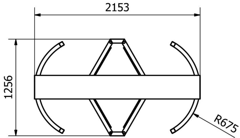
GENERAL DIMENTIONS
