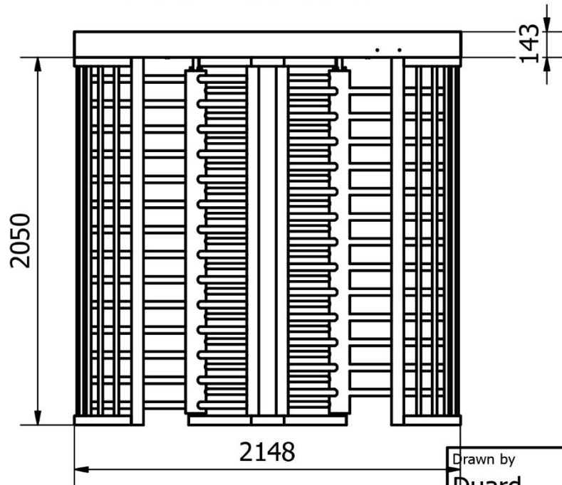
GENERAL DIMENTIONS
