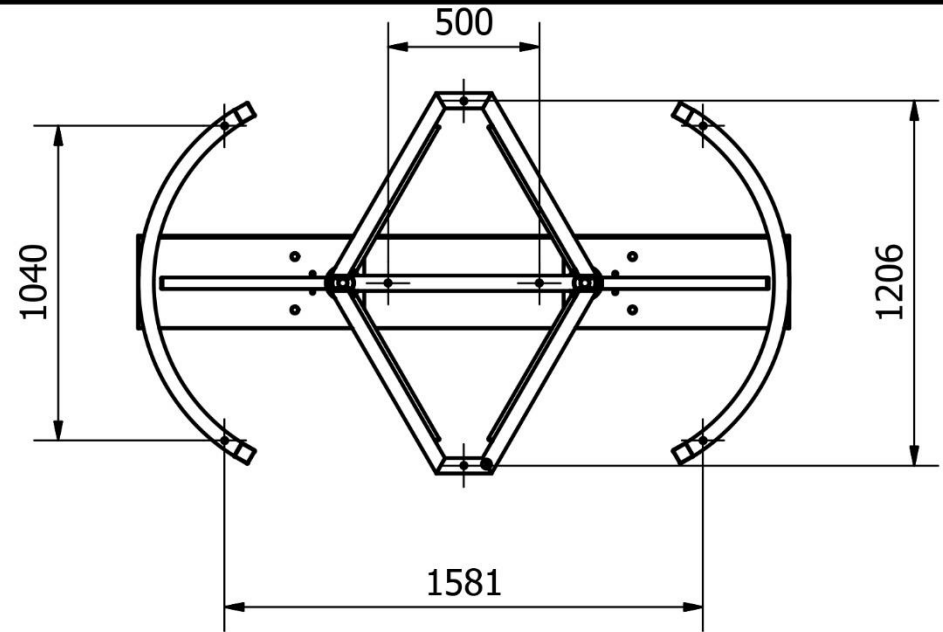
MOUNTING DIMENTIONS
